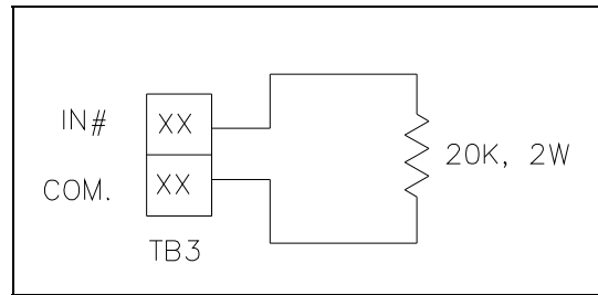
Figure 5. Unused Input
