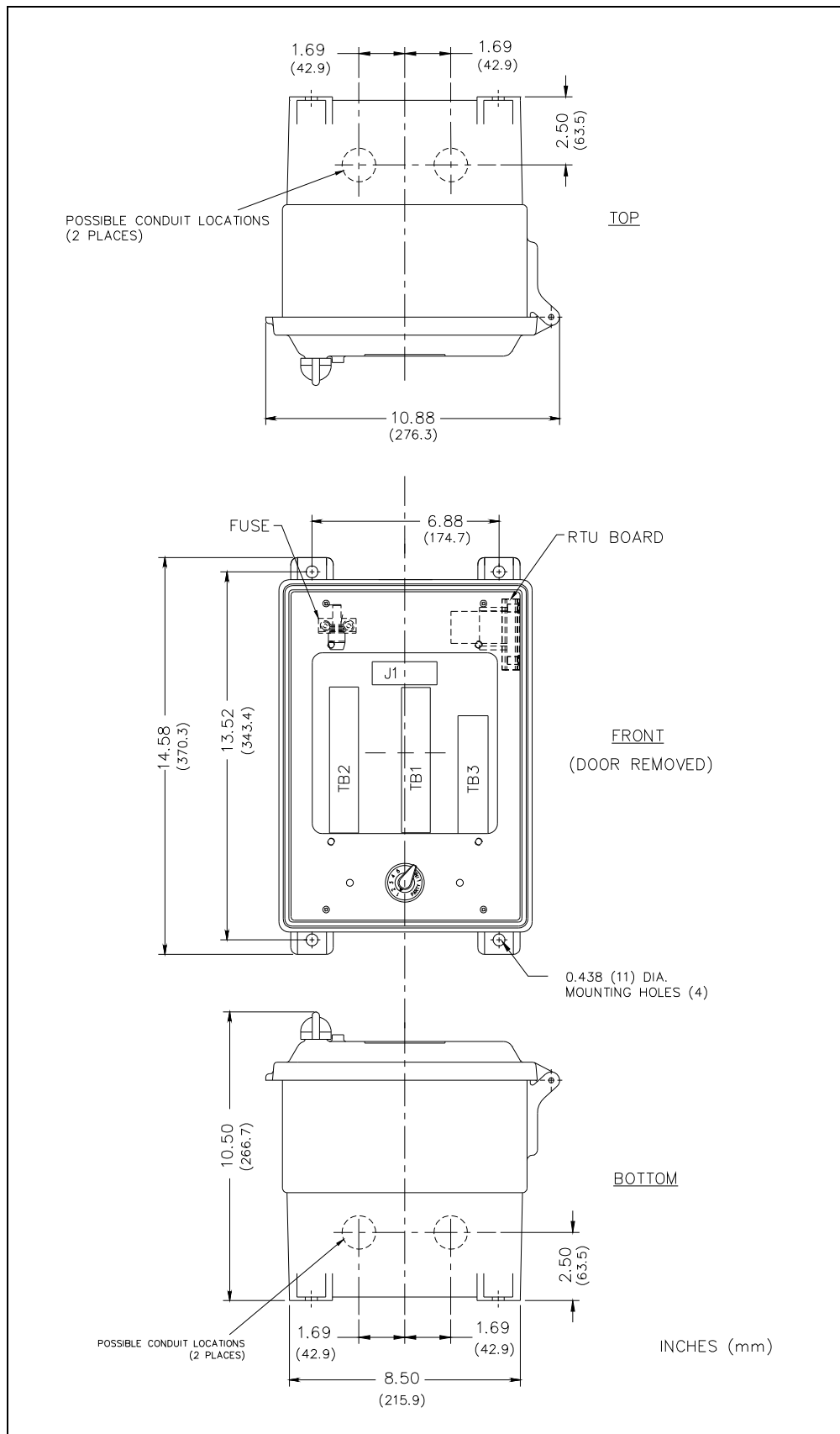
Figure 6. Model 7335-005 SmartSeries® Outdoor Non-Metallic RTU Enclosure
